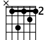
Bm7
