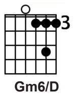
Gm6/D
