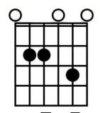
Em7
