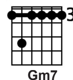
Gm7
