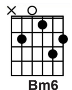
Bm6
